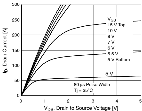
Figure 9. Saturation Characteristics
