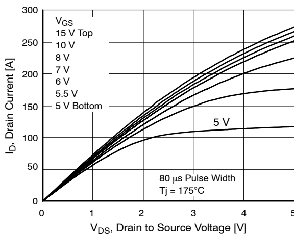
Figure 10. Saturation Characteristics
