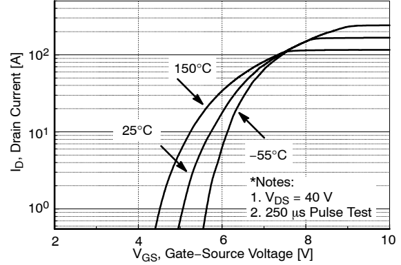
Figure 2. Transfer Characteristics
