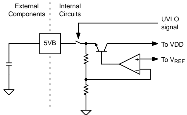
Figure 17. 5 V Bias
