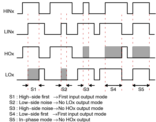
Figure 40. Interlock Function
