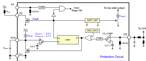
Figure 42. Over-Current Protection
