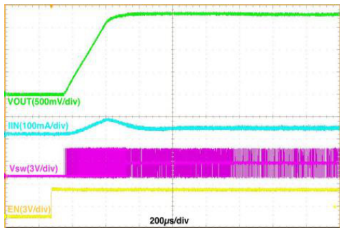
Figure 20. Start-up, V_{IN} = 3.6\text{ V} , V_{OUT} = 1.8\text{ V} , 50 mA Resistive Load, Auto Mode
