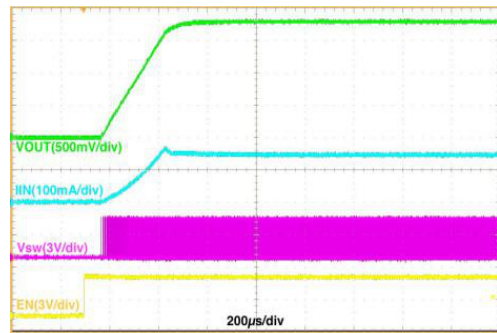
Figure 21. Start-up, V_{IN} = 3.6\text{ V} , V_{OUT} = 1.8\text{ V} , 300 mA Resistive Load, Auto Mode
