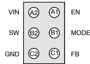
Figure 3. Bottom View
