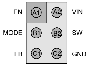
Figure 2. Top View
