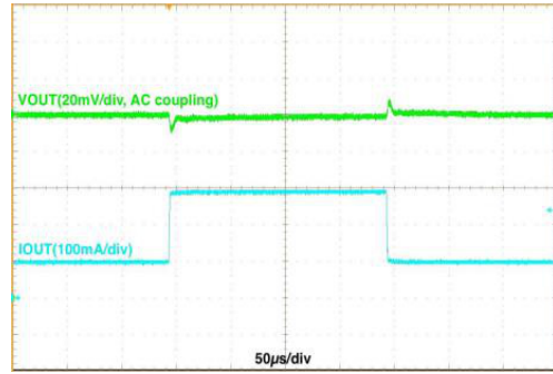
Figure 17. Load Transient, V_{IN} = 3.6\text{ V} , V_{OUT} = 1.8\text{ V} , 100 mA \leftrightarrow 300 mA, 1 \mu\text{s} Edge, Auto Mode
