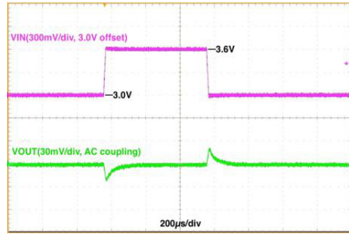
Figure 19. Line Transient, V_{IN} = 3.0\text{ V} \leftrightarrow 3.6\text{ V} , V_{OUT} = 1.8\text{ V} , 10 \mu\text{s} Edge, 300 mA Load, Auto Mode
