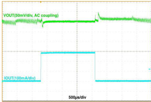
Figure 16. Load Transient, V_{IN} = 3.6\text{ V} , V_{OUT} = 1.8\text{ V} , 5 mA \leftrightarrow 300 mA, 1 \mu\text{s} Edge, Auto Mode
