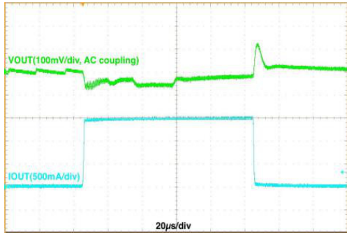
Figure 18. Load Transient, V_{IN} = 3.6\text{ V} , V_{OUT} = 1.8\text{ V} , 10 mA \leftrightarrow 1500 mA, 1 \mu\text{s} Edge, Auto Mode
