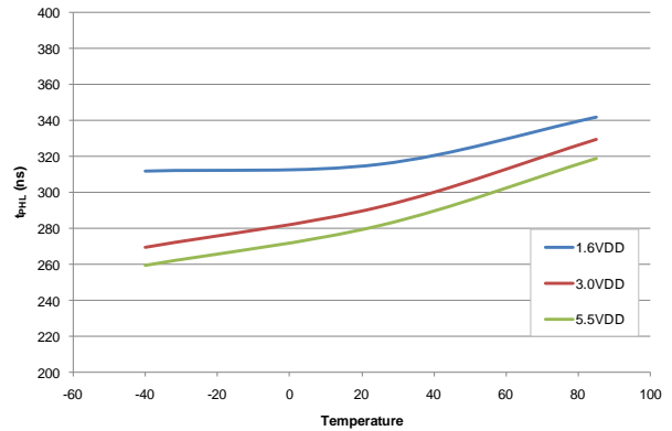
Figure 9. Propagation Delay (t PL ) vs. Temperature
