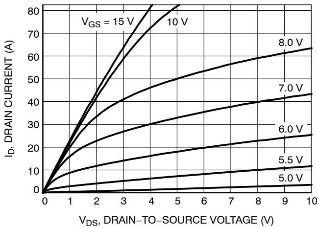
Figure 9. Saturation ( 25^\circ\text{C} )
