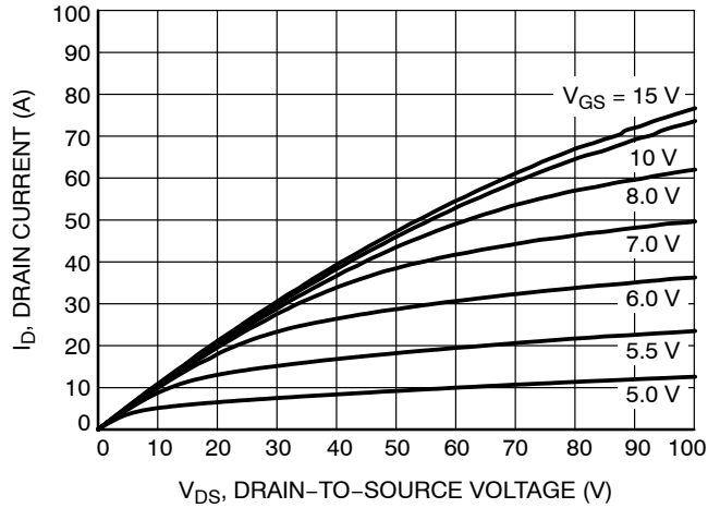
Figure 10. Saturation ( 150^\circ\text{C} )
