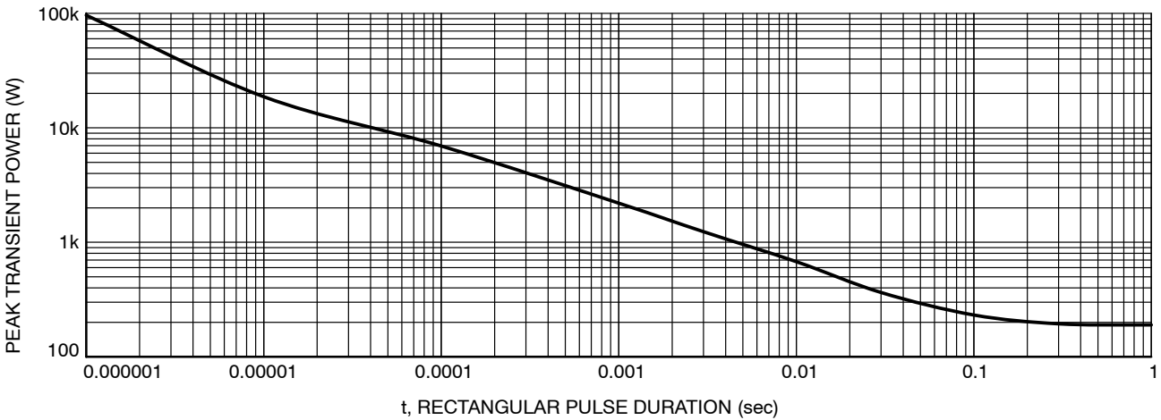
Figure 20. Peak Power
