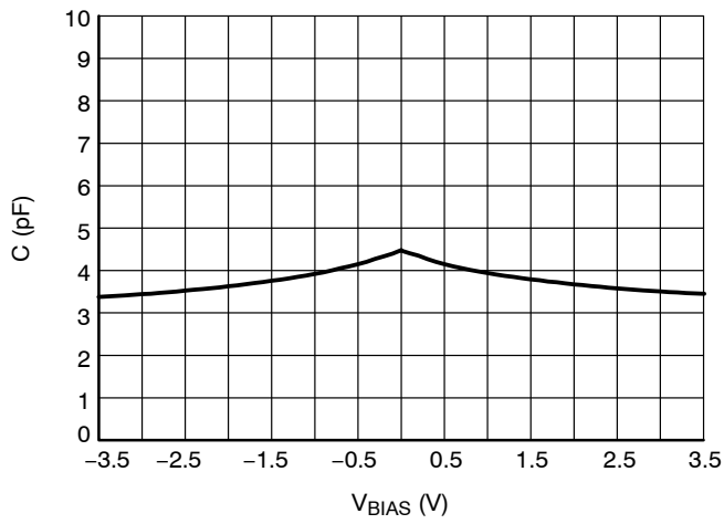
Figure 1. CV Characteristics
