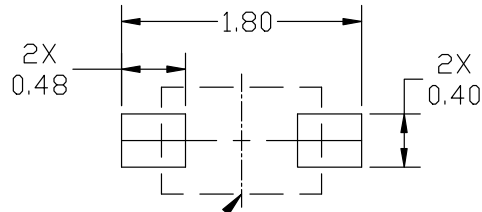
PACKAGE OUTLINE
