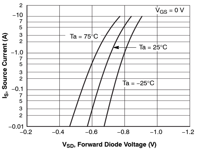
Figure 7. I_S - V_{SD}
