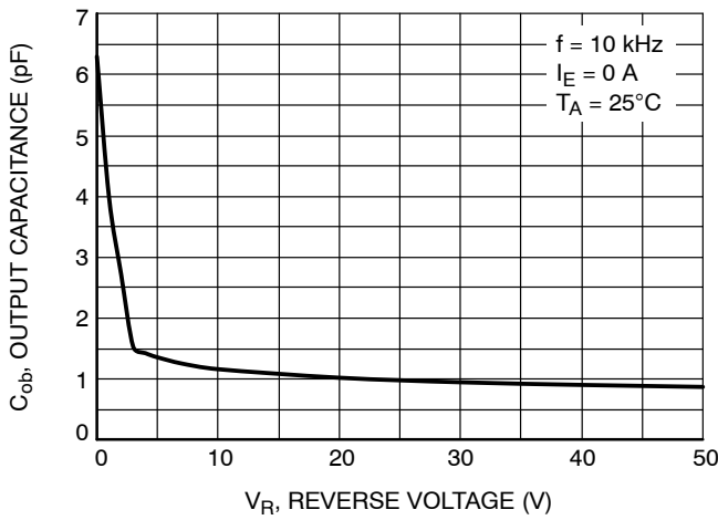
Figure 19. Output Capacitance
