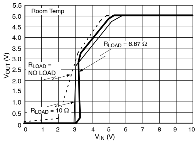
Figure 5. V OUT vs. V IN Over R LOAD
