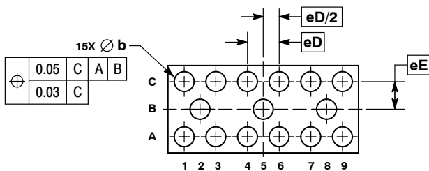
BOTTOM VIEW
