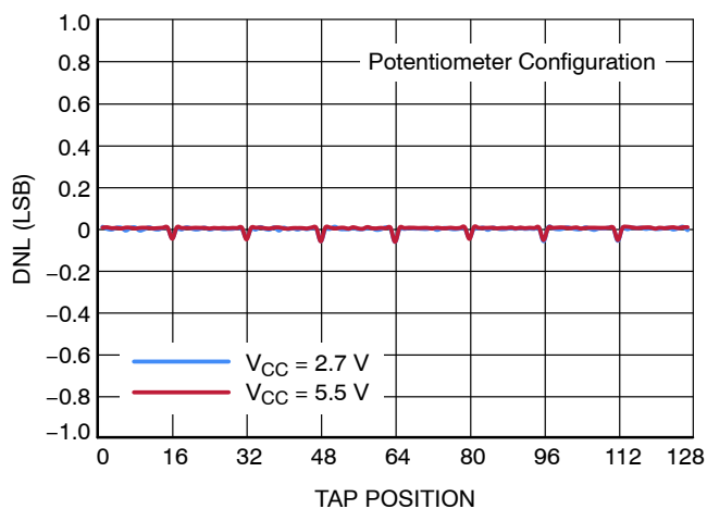
Figure 5. Differential Non-Linearity
