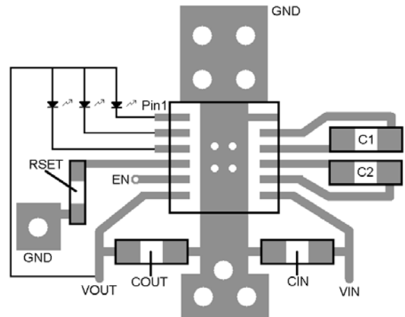
Figure 22. Recommended Layout
