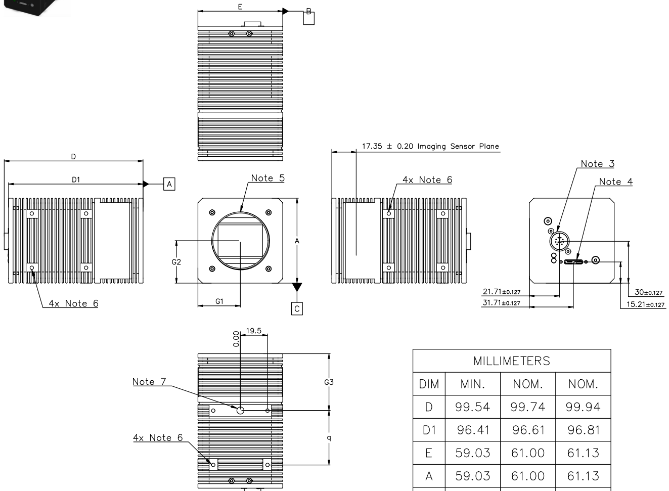
CMOD 99.74x61.00x61.00 CASE 810AB ISSUE A
