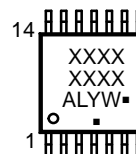
TSSOP-14 DT SUFFIX CASE 948G
