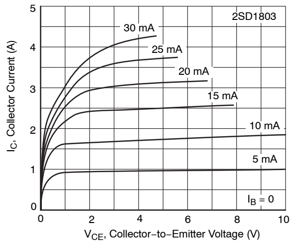
Figure 4. I_C - V_{CE}
