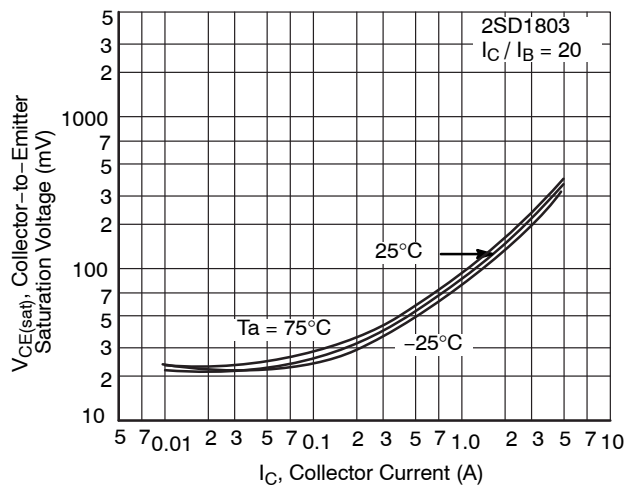
Figure 14. V_{CE(sat)} - I_C
