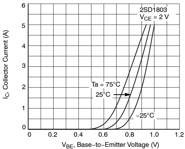
Figure 6. I_C - V_{BE}
