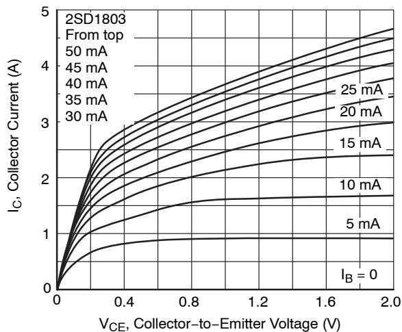
Figure 2. I_C - V_{CE}
