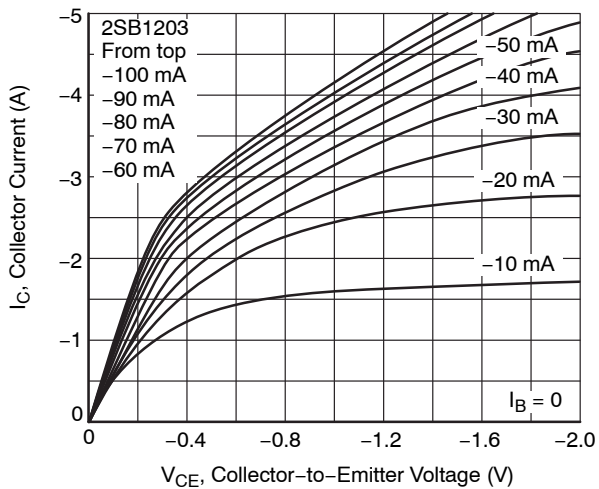
Figure 1. I_C - V_{CE}
