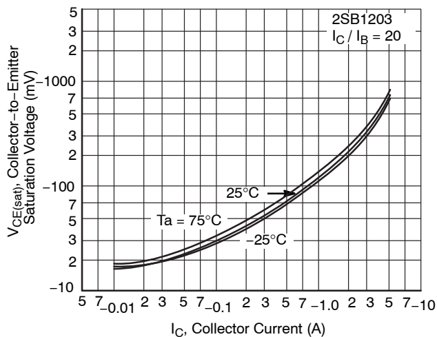
Figure 13. V_{CE(sat)} - I_C
