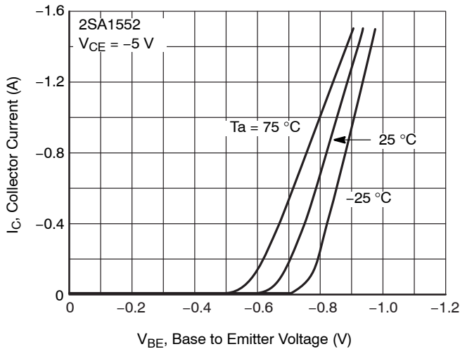
Figure 6. I_C - V_{BE}
