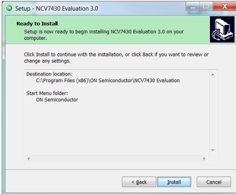
Figure 13 - Install DLL
