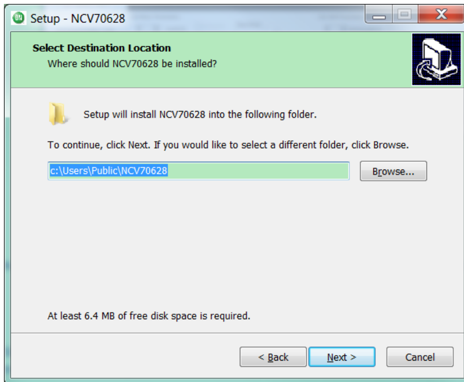
Figure 6 - Select Destination
