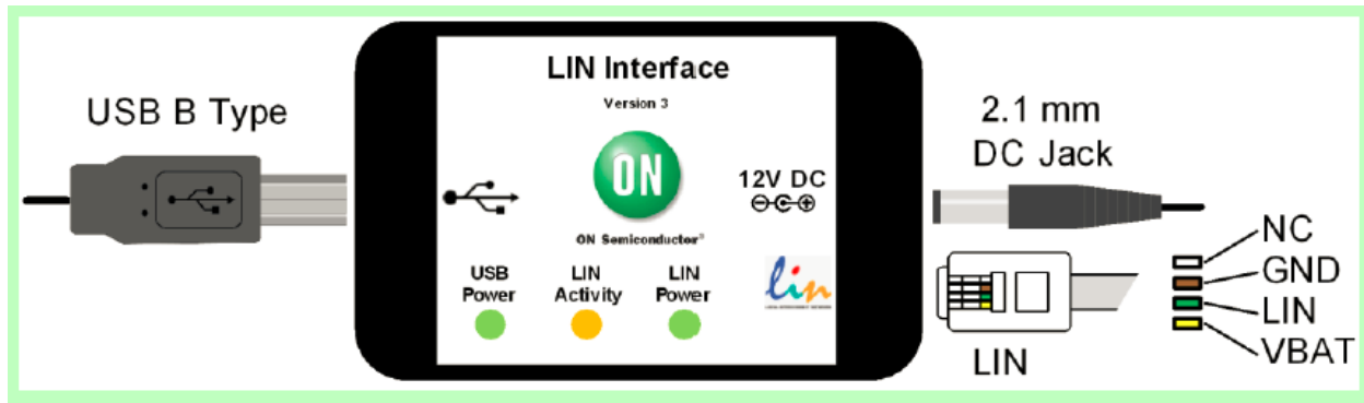
Figure 2 - USB to LIN Interface Connectors
