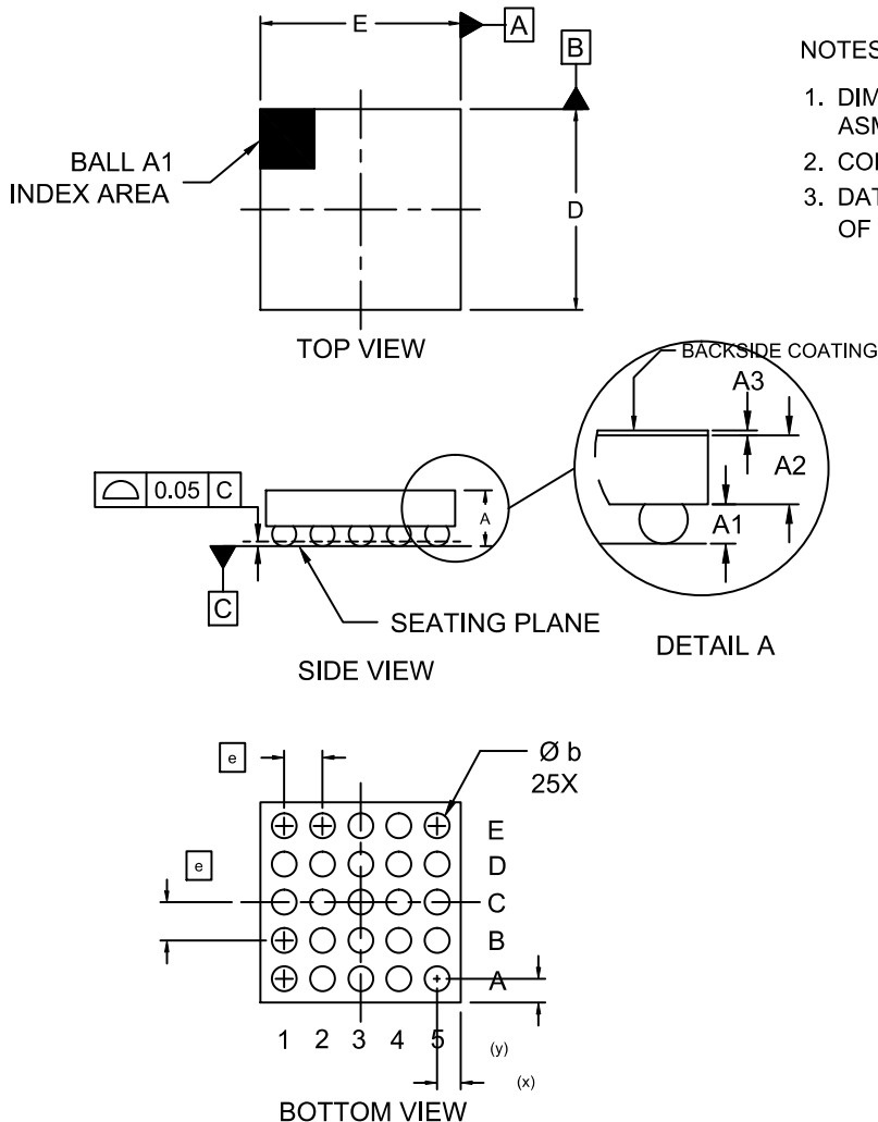
WLCSP25 2.16x2.16x0.574 CASE 567YL ISSUE O
