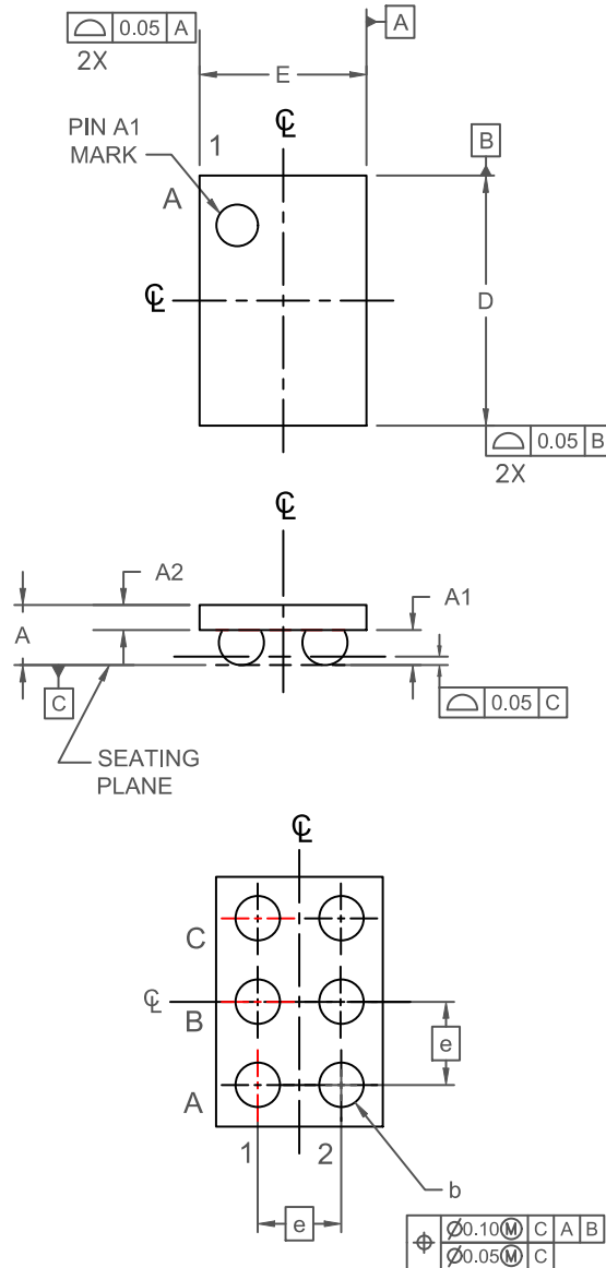
WLCSP6 1.0x1.5x0.4 CASE 567PT ISSUE A
