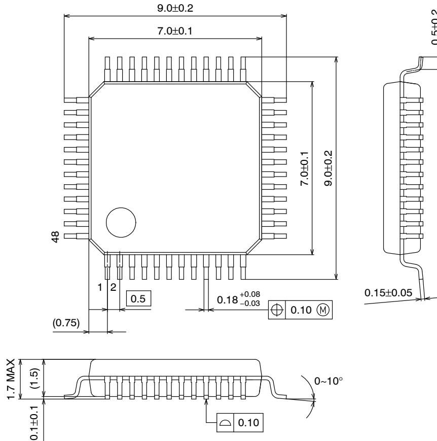
SPQFP48 7x7 / SQFP48 CASE 131AJ ISSUE A
