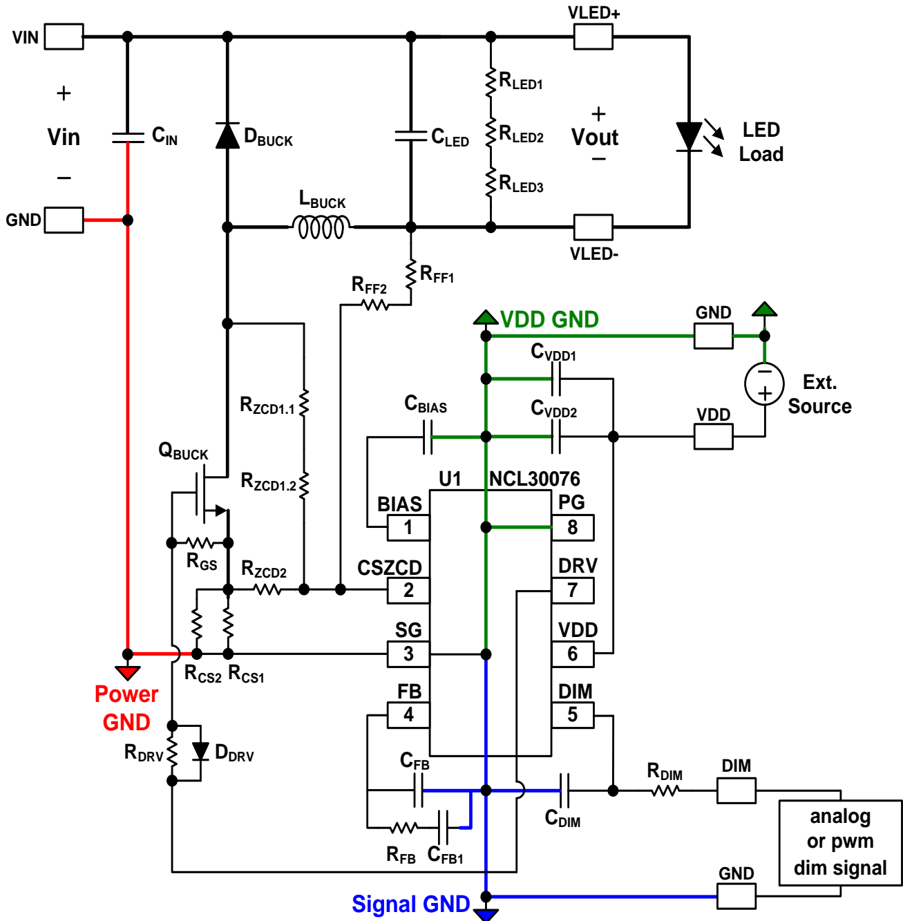
Figure 1. Schematic for NCL30076 100-W Design Reference
