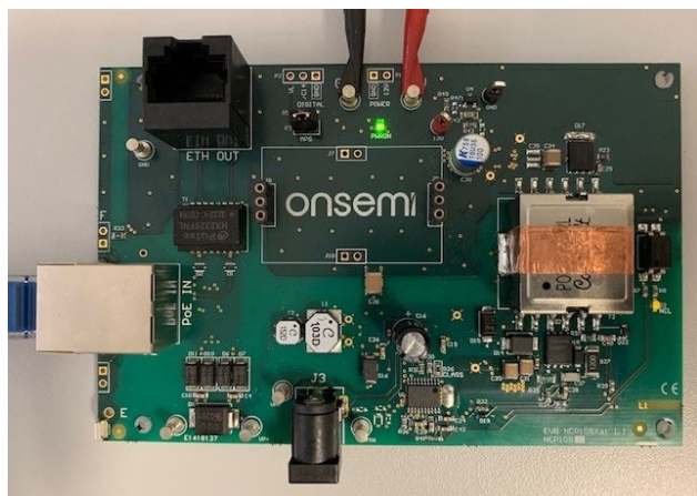
Figure 1. Operational NCP1081REF12VC4GEVB showing Basic Interconnections
