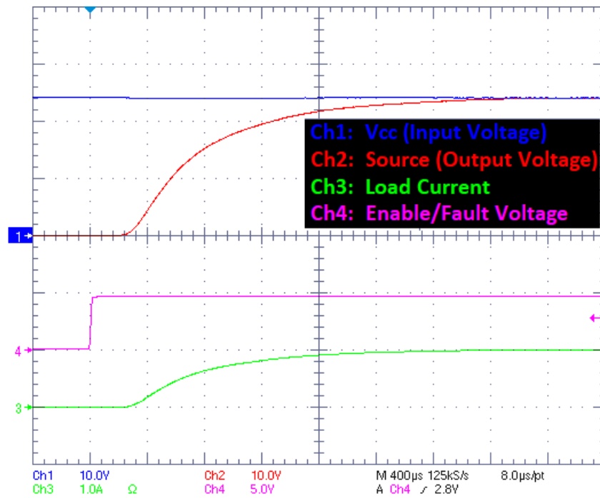
Figure 3. Hot Plug with dvdt Open into 24 Ω Load (400 µs/Division Timescale)
