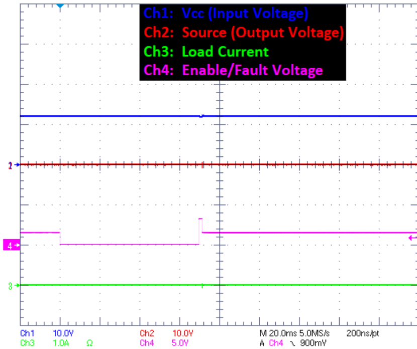
Figure 8. Drawing Current with an Electronic Load, Showing the Overload ( I_{OL} ) and Short Circuit ( I_{SC} ) Current Limits
