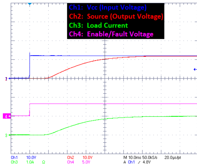
Figure 4. Hot Plug into 12 \Omega Load with CdvdT of 2.2 nF engaged to show Slower Controlled Output Voltage Ramp
