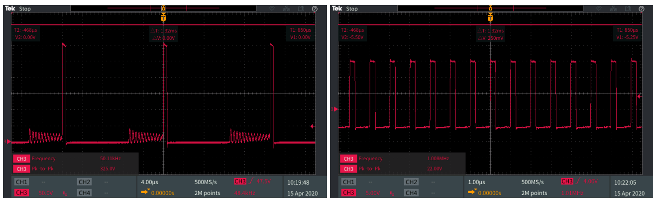
Figure 27. Switching Waveform of +15 V Buck Converter (U50) and –5 V Buck–Boost Converter (U60)
