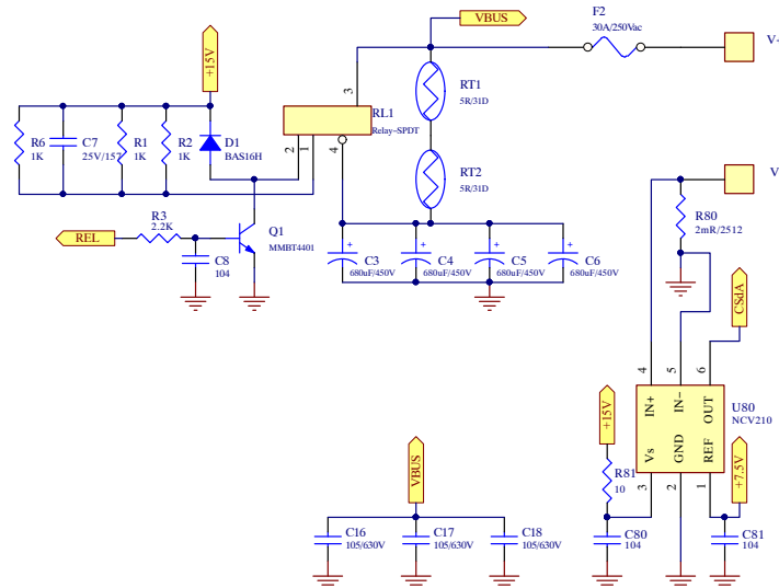
Figure 12. Schematic of the Inrush Current Limit and DC Terminal Current Sense
