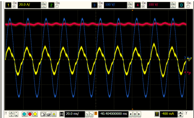
Figure 23. Vin 220 V, Pin = 3.3 kW
