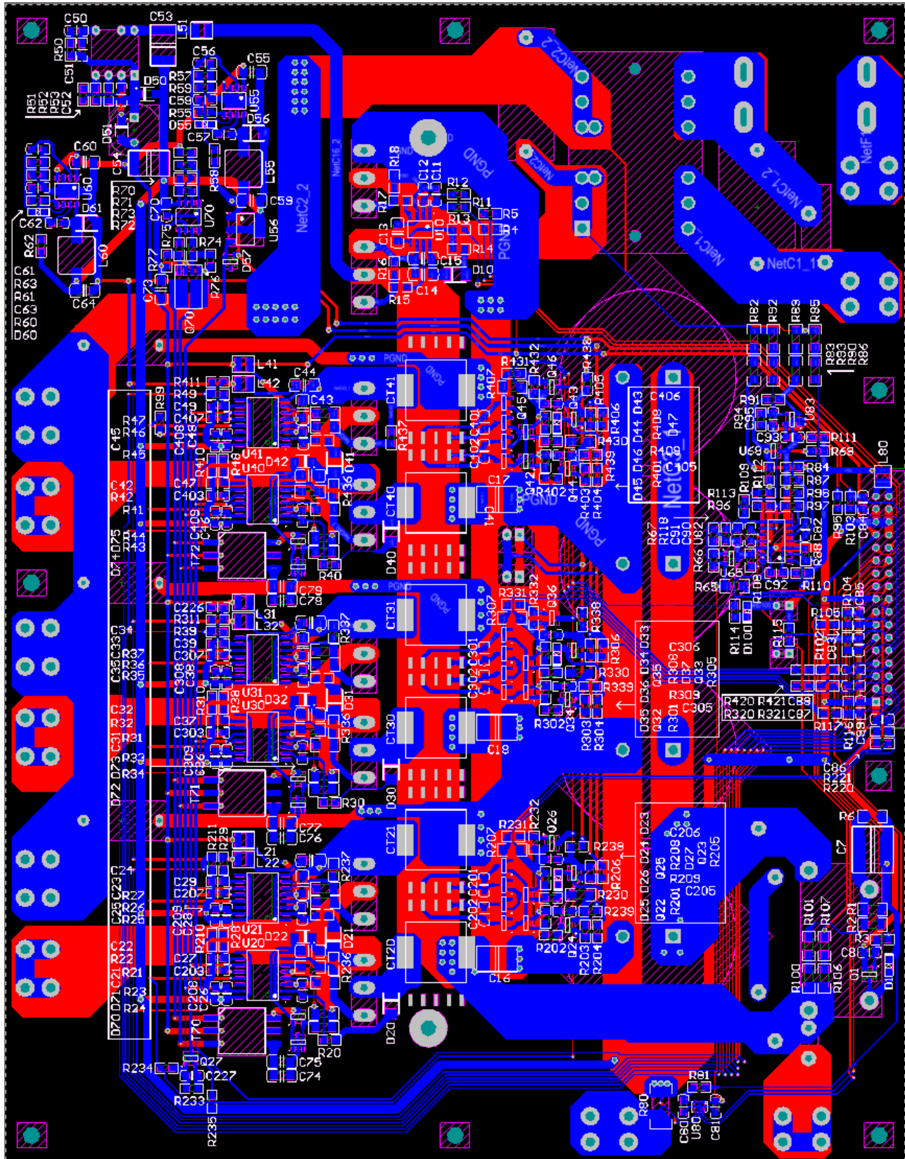
Figure 34. Bottom Side View of Main Board
