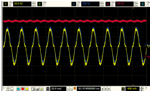
Figure 22. Vin 120 V, Pin = 3.3 kW
