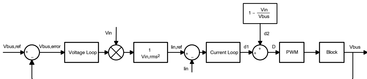
Figure 15. Voltage Loop and Current Loop Control Model
