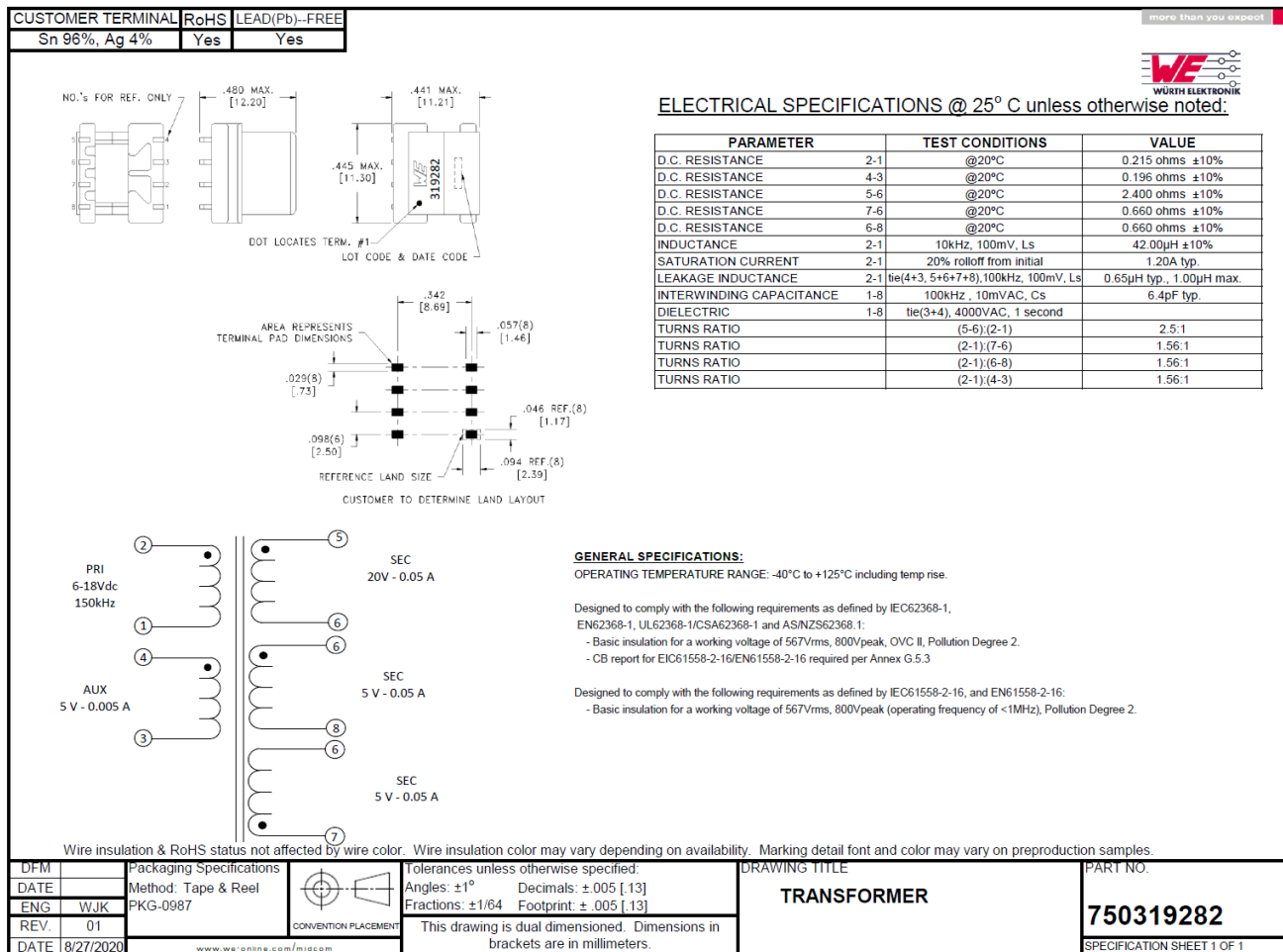
Figure 13. Drawing and Parameters of Used Transformer
