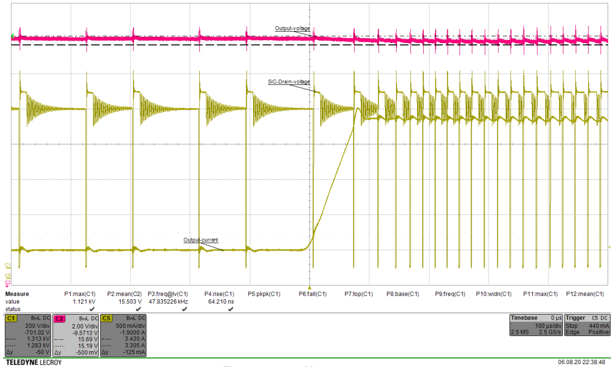
Figure 16. 900 V – 15% to 85%
