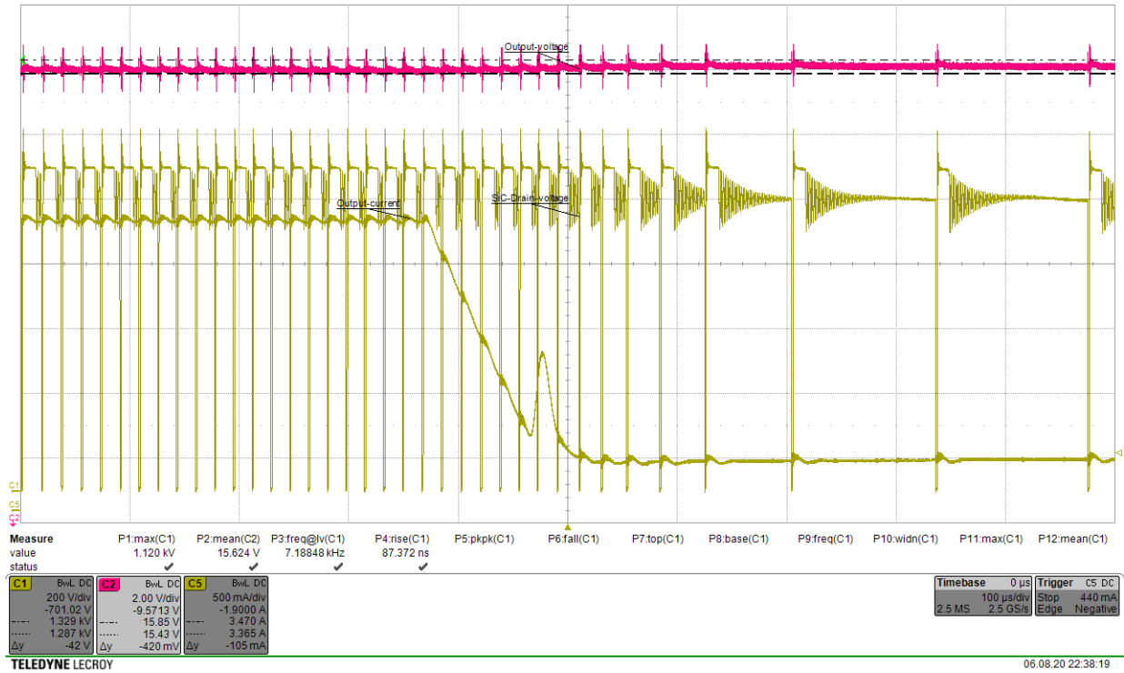
Figure 17. 900 V – 85% to 15%
