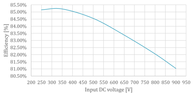
Efficiency 40W HV Auxiliary
