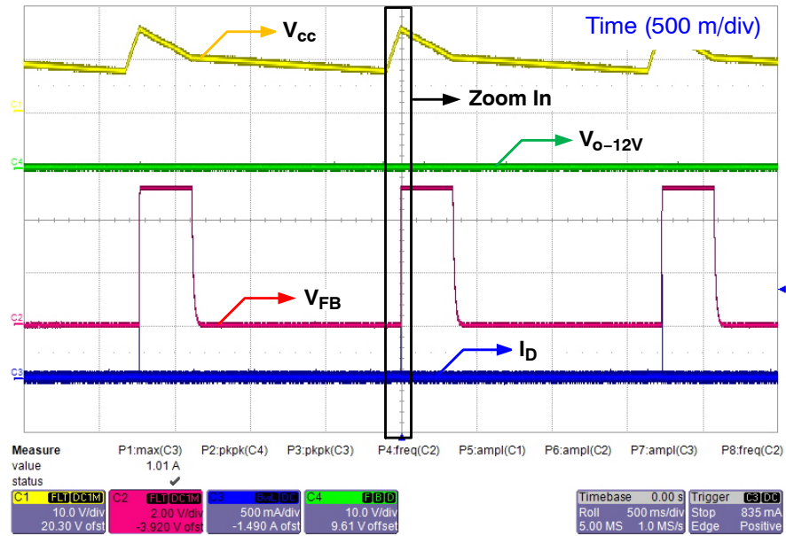
Figure 35. CSSP @ 230 V_{ac} /60 Hz, Full Load (Roll Mode)
