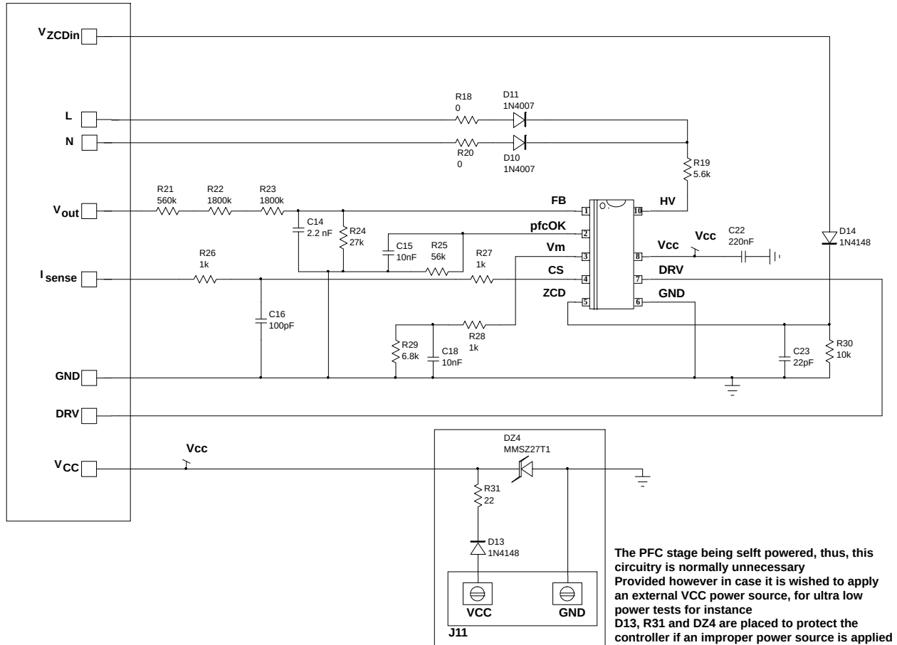
Figure 3. Control Section of the Application Schematic
