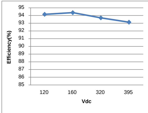
At 75% load
