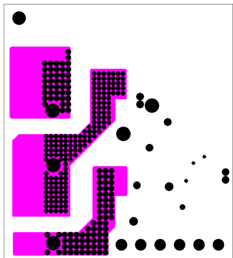
Layer 3, Internal
