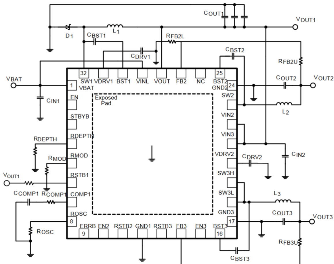
Figure 3. Typical Application
