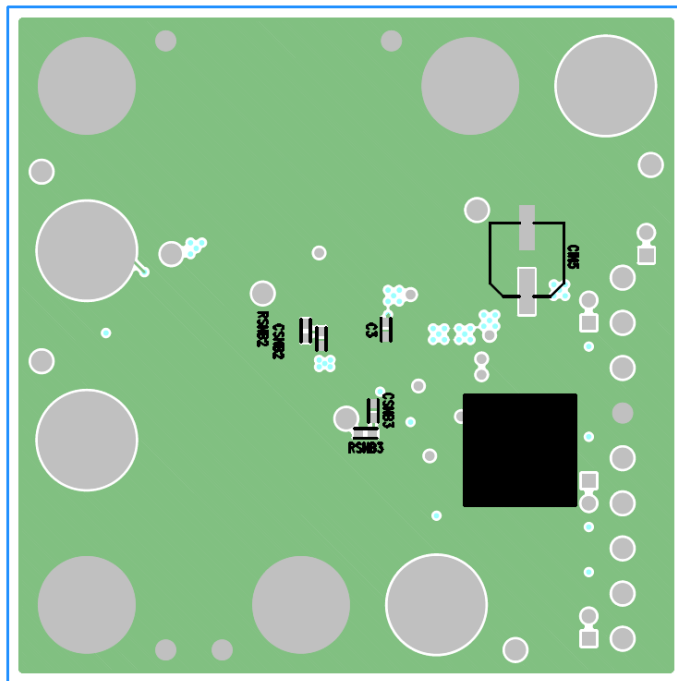
Figure 16. Bottom View
