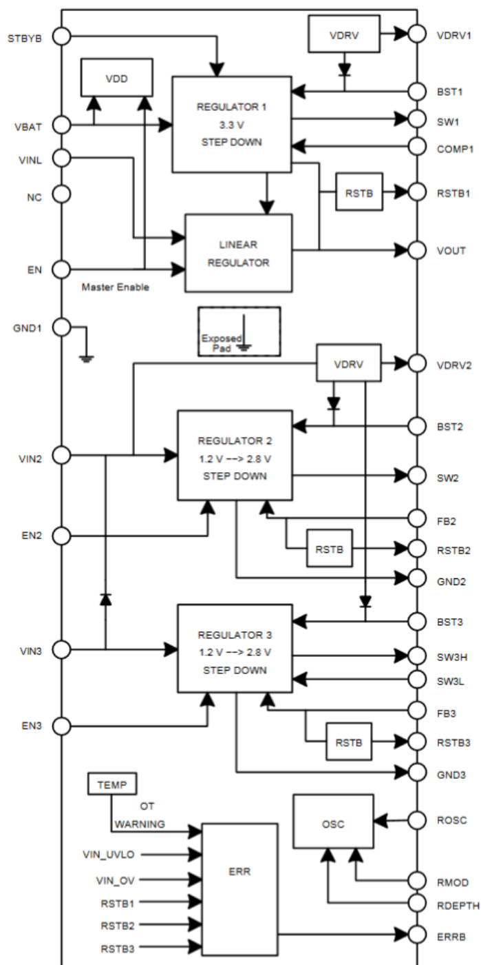
Figure 2. NCV97310A Block Diagram
