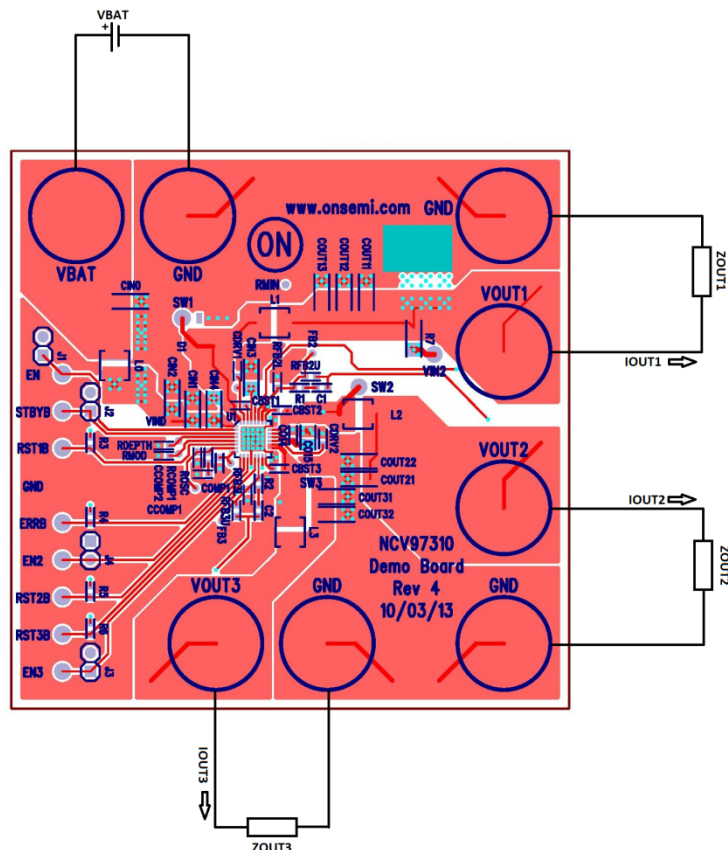
Figure 5. NCV97310A Board Connections
