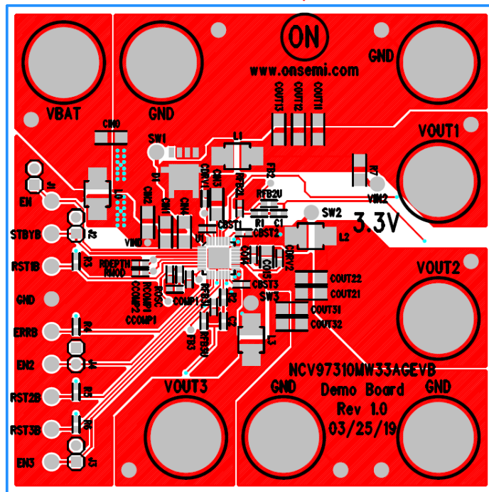
Figure 15. Top View
