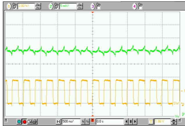
Figure 5. Typical Operation Waveforms of NCV6323C/D Evaluation Board
