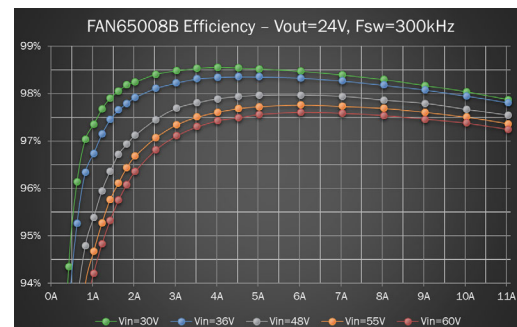
Figure 2. FAN65008B Efficiency
