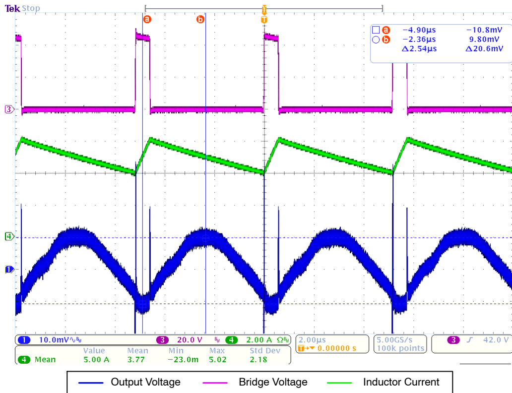
Figure 18. Output Voltage Ripple I_{\text{OUT}} = 5 \text{ A}
