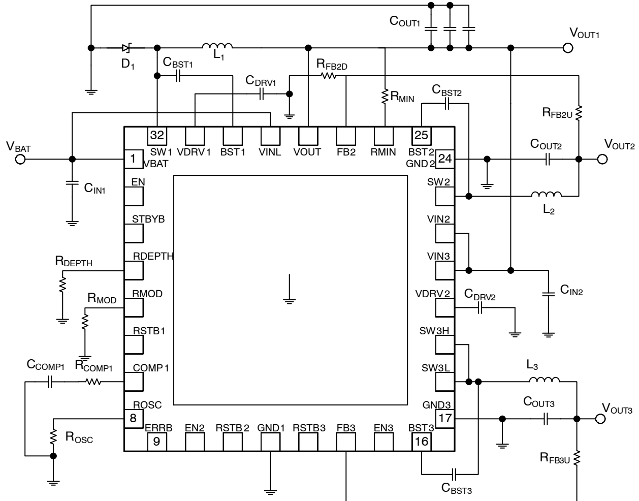
Figure 3. Typical Application
