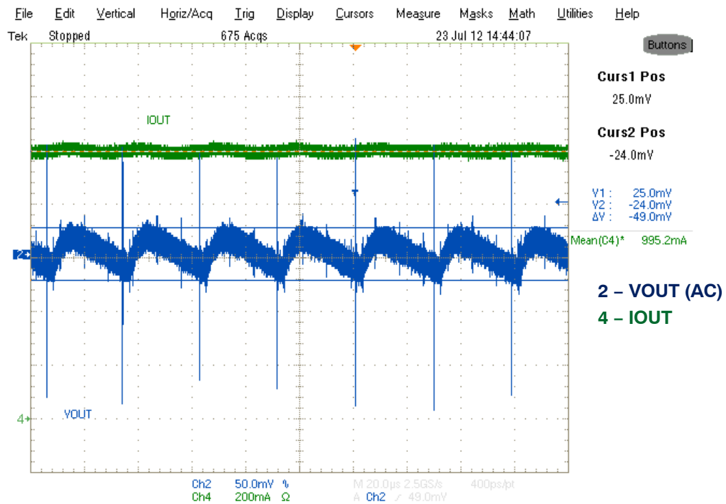
Figure 7. V_{IN} = 230\text{ V}_{AC} , I_{OUT} = 1.0\text{ A} , \Delta V_{OUTPK-PK} = 50\text{ mV}
