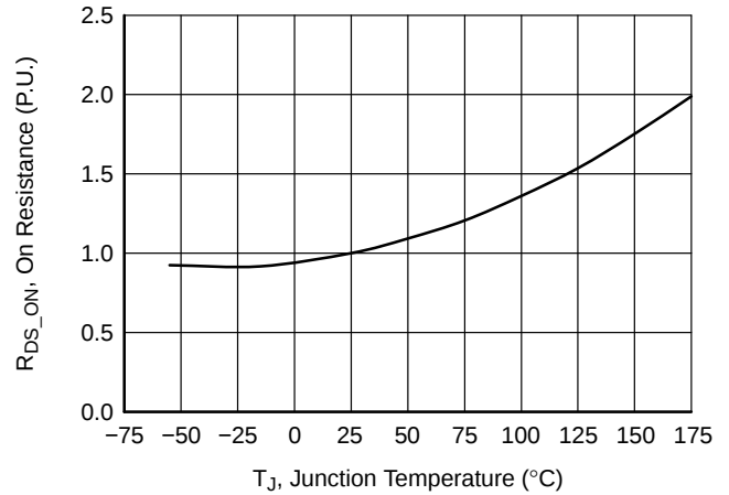
Figure 4. Normalized On-Resistance vs. Temperature at V_{GS} = 12 V and I_D = 100 A
