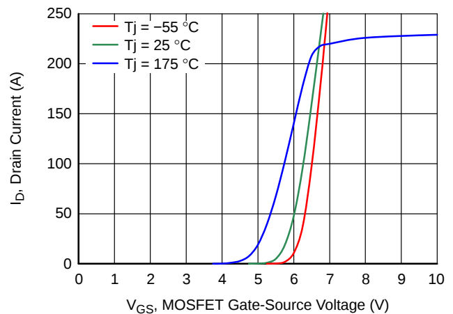
Figure 6. Typical Transfer Characteristics at V_{DS} = 5 V
