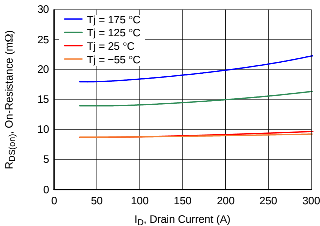
Figure 5. Typical Drain-Source On-Resistances at V_{GS} = 12 V
