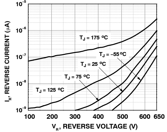
Figure 3. Reverse Characteristics
