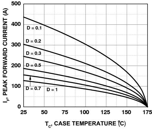
Figure 4. Current Derating
