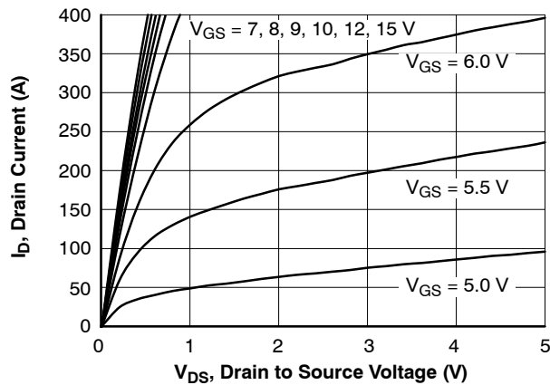
Figure 5. Saturation Characteristics
