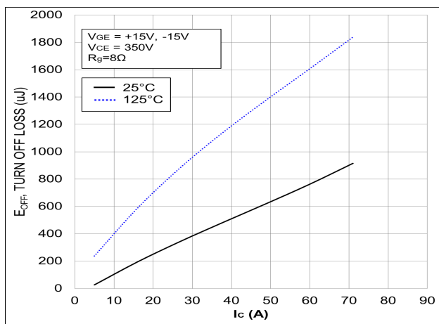
Figure 19. Typical Switching Loss E_{OFF} vs. I_C
