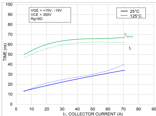
Figure 23. Typical Switching Time T_{DON} vs. I_C
