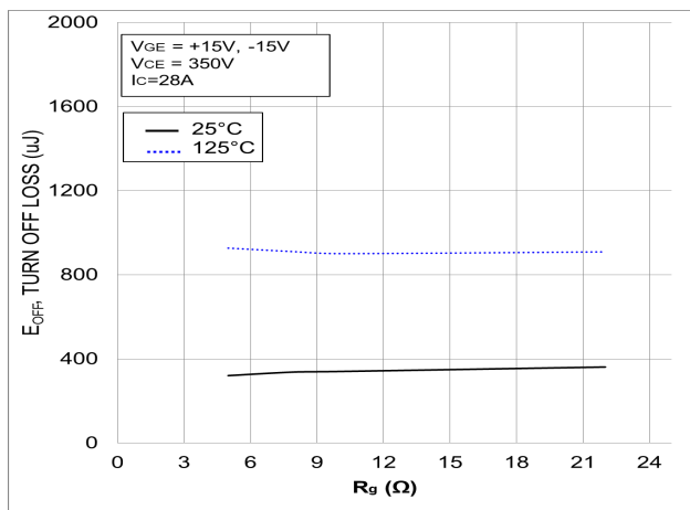
Figure 21. Typical Switching Loss E_{OFF} vs. R_g
