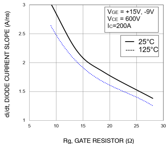
Figure 33. Typical di/dt vs. Rg
