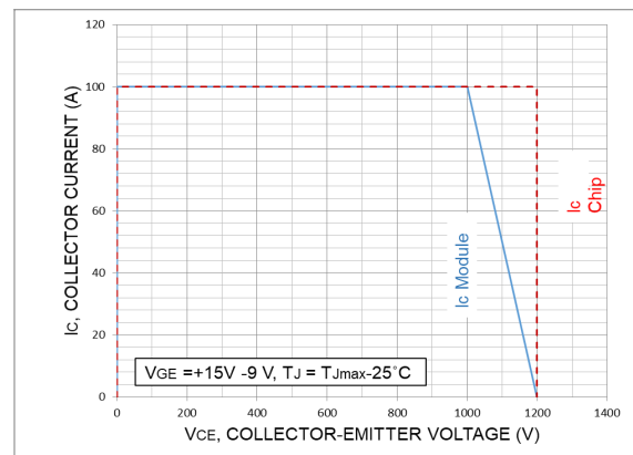
Figure 7. RBSOA
