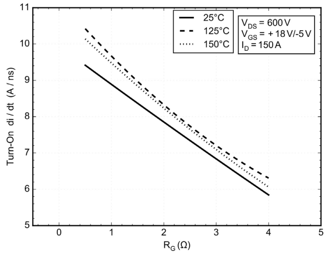
Figure 23. di/dt ON vs. R_G
