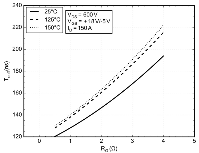
Figure 17. Typical Switching Loss T_{doff} vs. R_G
